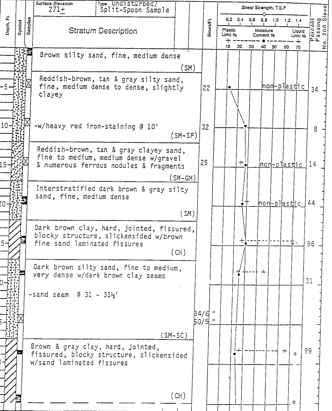
LOG OF BORING NO. B-2
