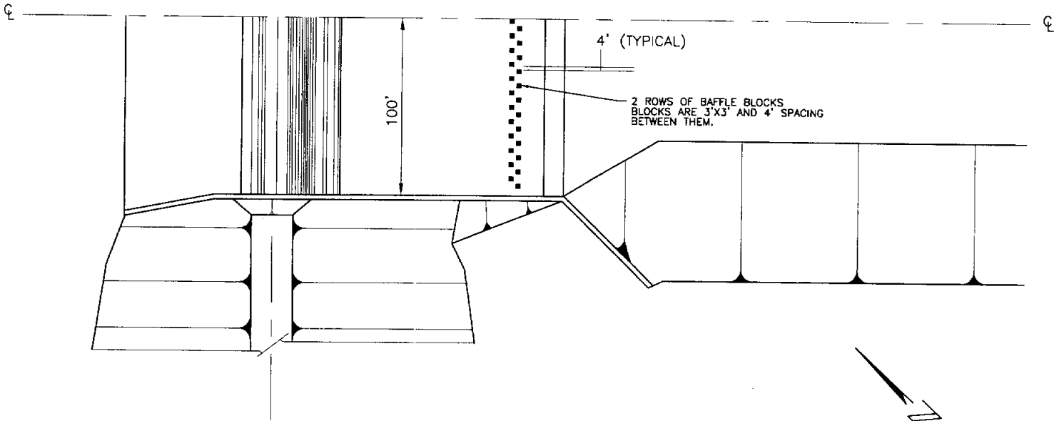
SERVICE SPILLWAY HALF-PLAN
