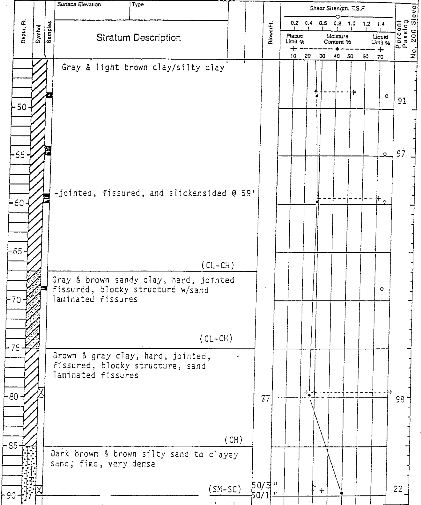
LOG OF BORING NO. 8-1 Cont.
