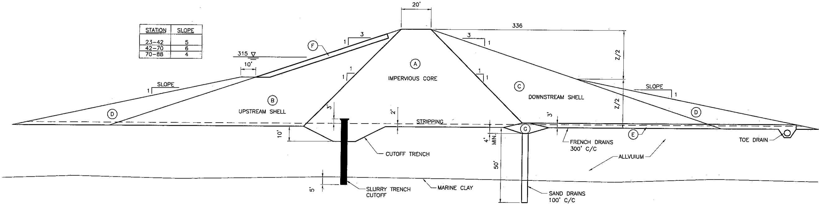
TYPICAL DAM SECTION SCALE: 1"=20'
