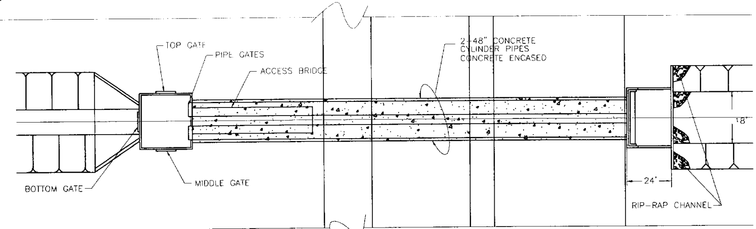
PLAN OF OUTLET WORKS
