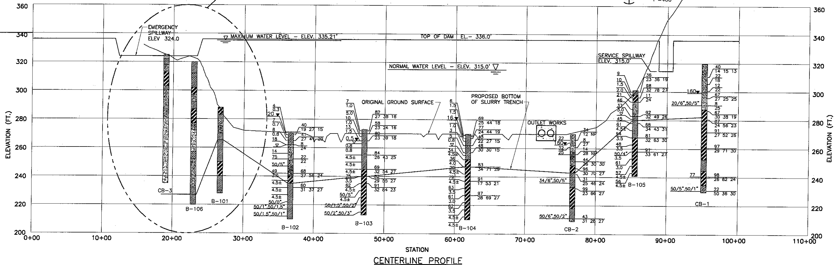
DETAIL 1"=400'
